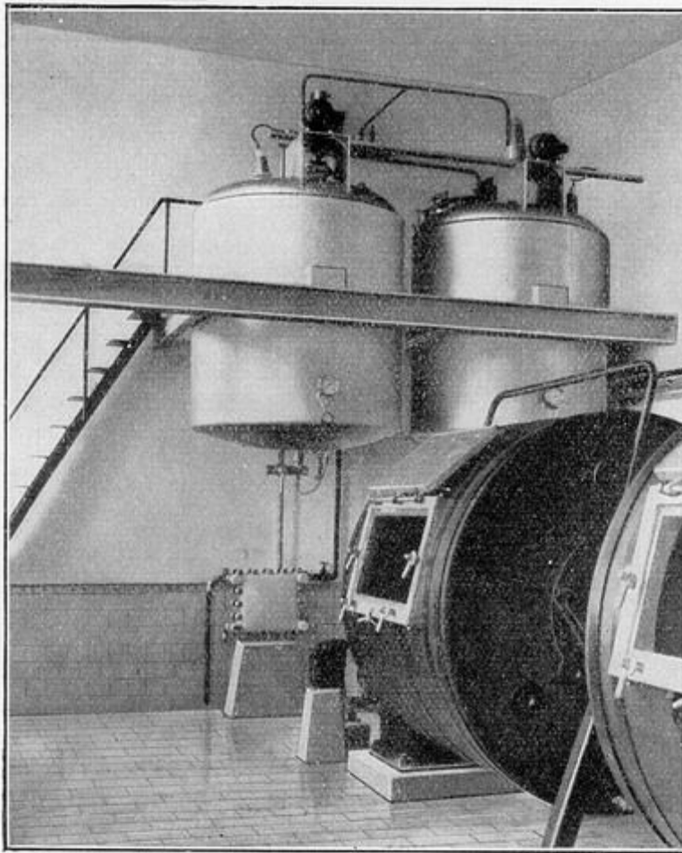
Fig. 52. Roomzuurtanks.
